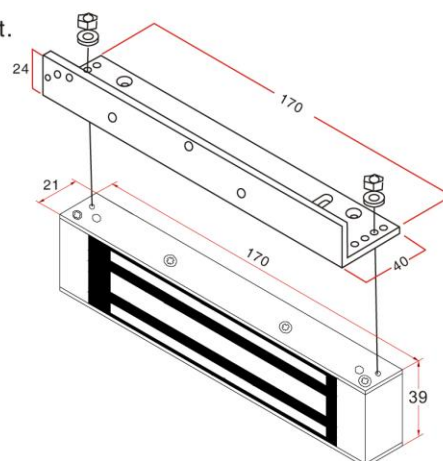
L Bracket Installation
