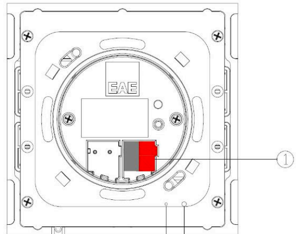
1. KNX Port Terminal 2. Programming Button 3. Programming LED
